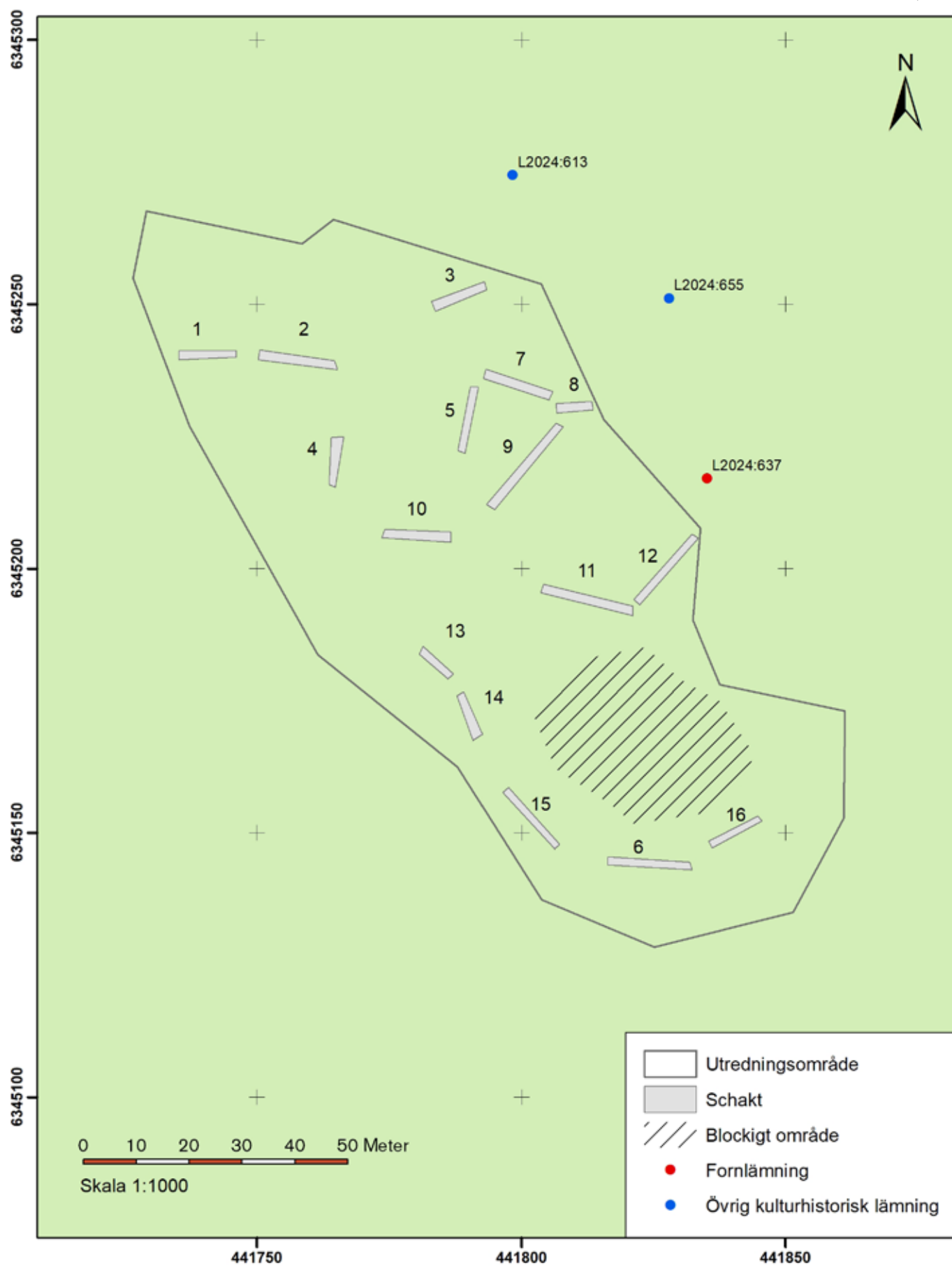
Figur 3. Schaktkarta, skala 1:1000
